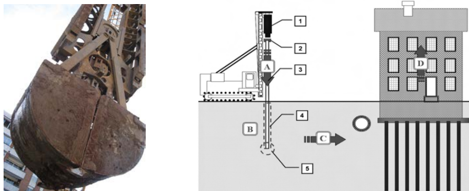
Construction machinery-induced ground vibrations problem.
