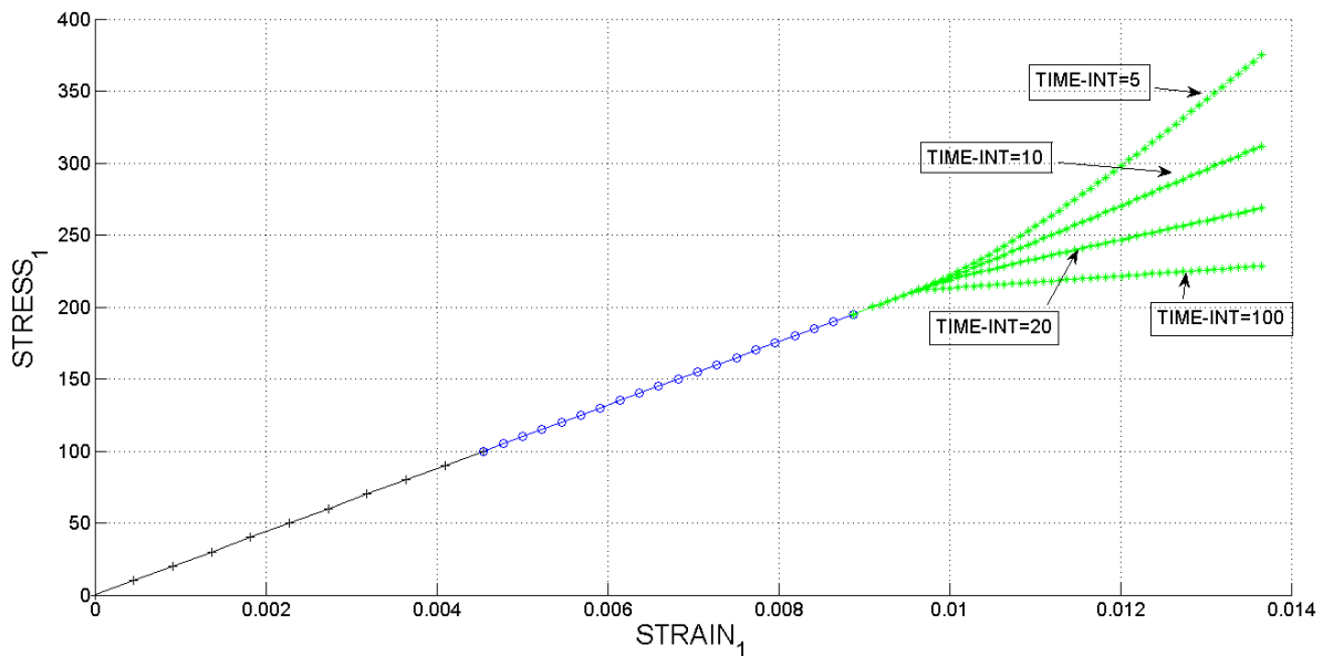
Figure 33. Strain1-Stress1 respect to strain rate
