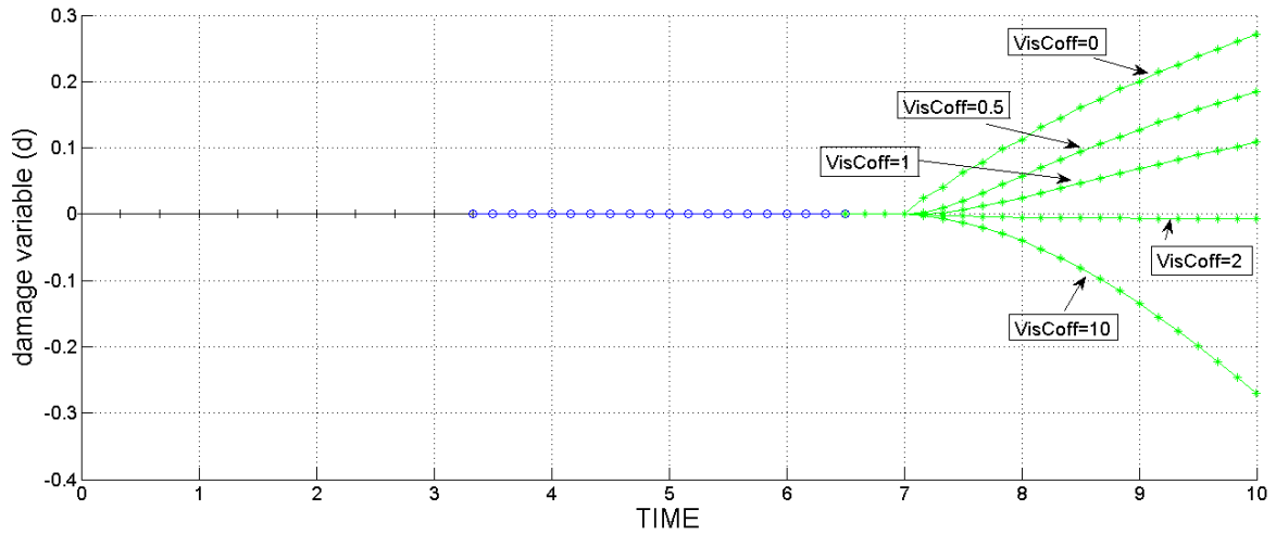
Figure 32. Damage variable respect to viscosity coefficient
