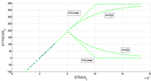
Figure 24. Strain1-Stress1 curve of case C
