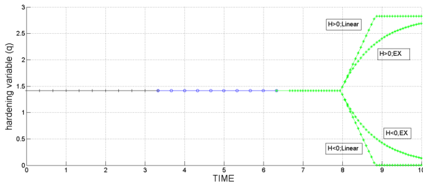
Figure 19. Hardening variable q respect to time of case A
