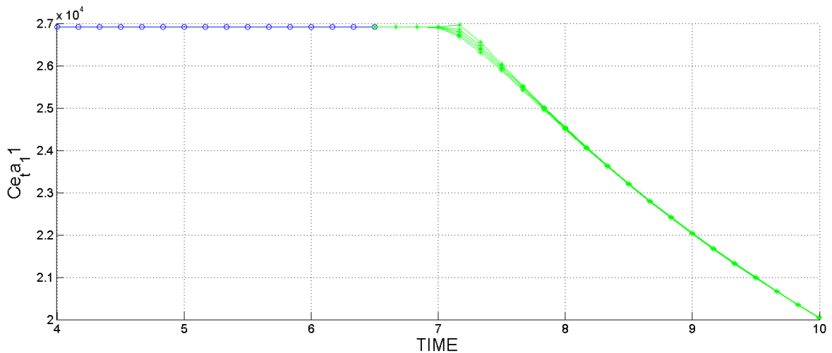
Figure 39. C11 component of tangent operator respect to \alpha when TIME-INT=10
