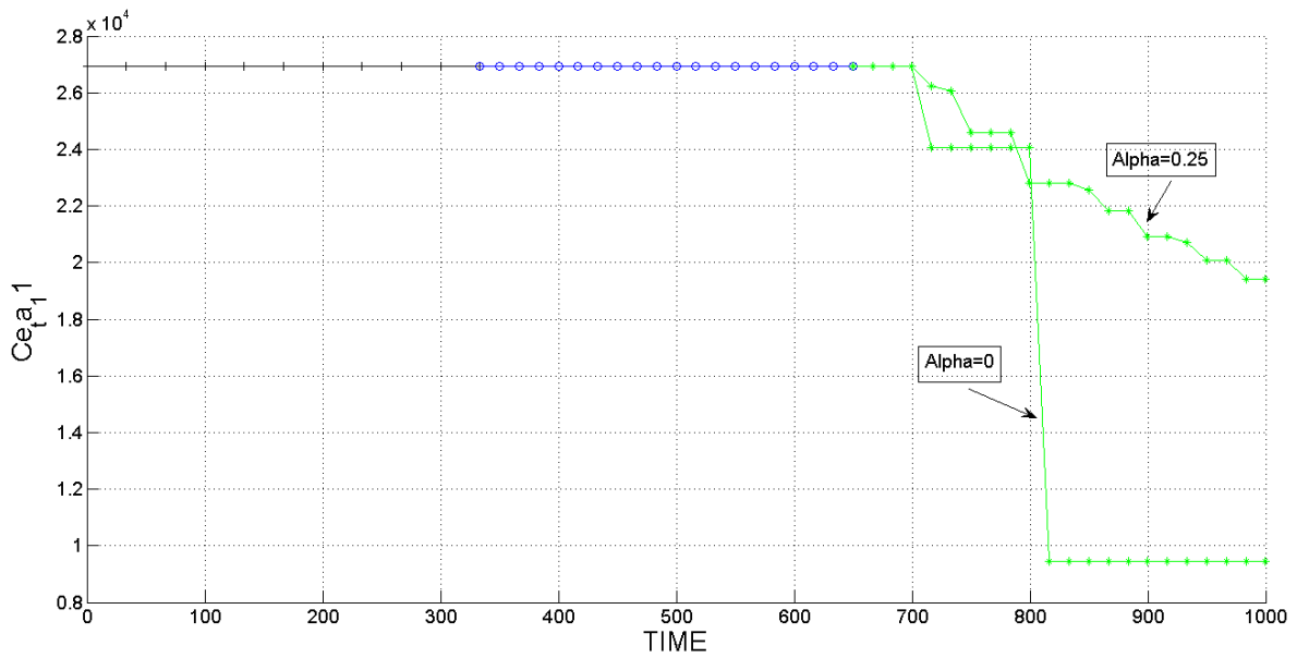
Figure 40. C11 component of tangent operator respect to \alpha when TIME-INT=1000 ( \alpha < 0.5 )
