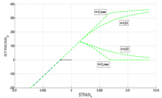
Figure 21. Strain2-Stress2 curve of case B
