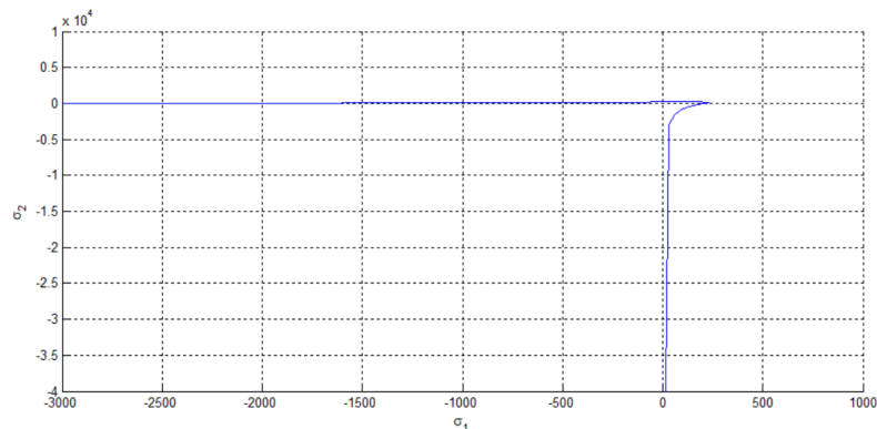
Figure 16. Tension-only model
