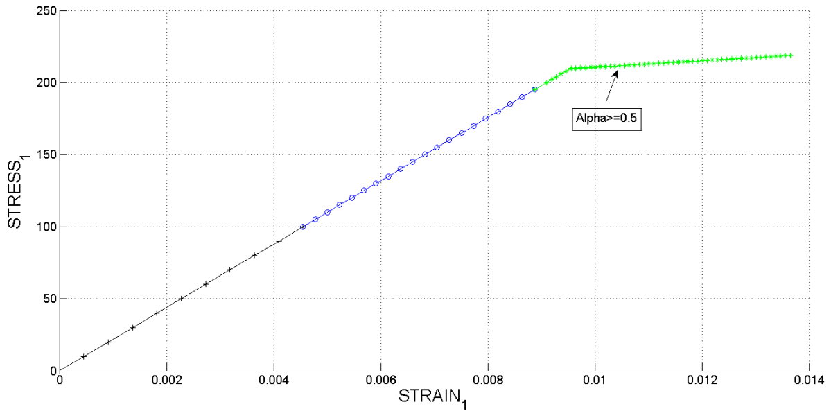
Figure 36. The Strain1-Stress1 respect to \alpha when TIME-INT=1000 ( \alpha \geq 0.5 )
