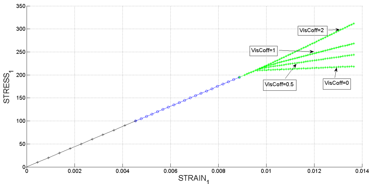
Figure 31. Strain1-Stress1 respect to viscosity coefficient
