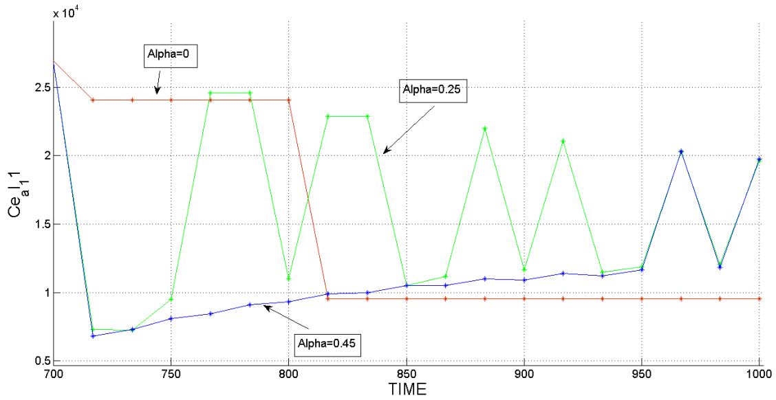
Figure 37. C11 component of algorithmic constitutive operator respect to \alpha when TIME-INT=1000 ( \alpha < 0.5 )
