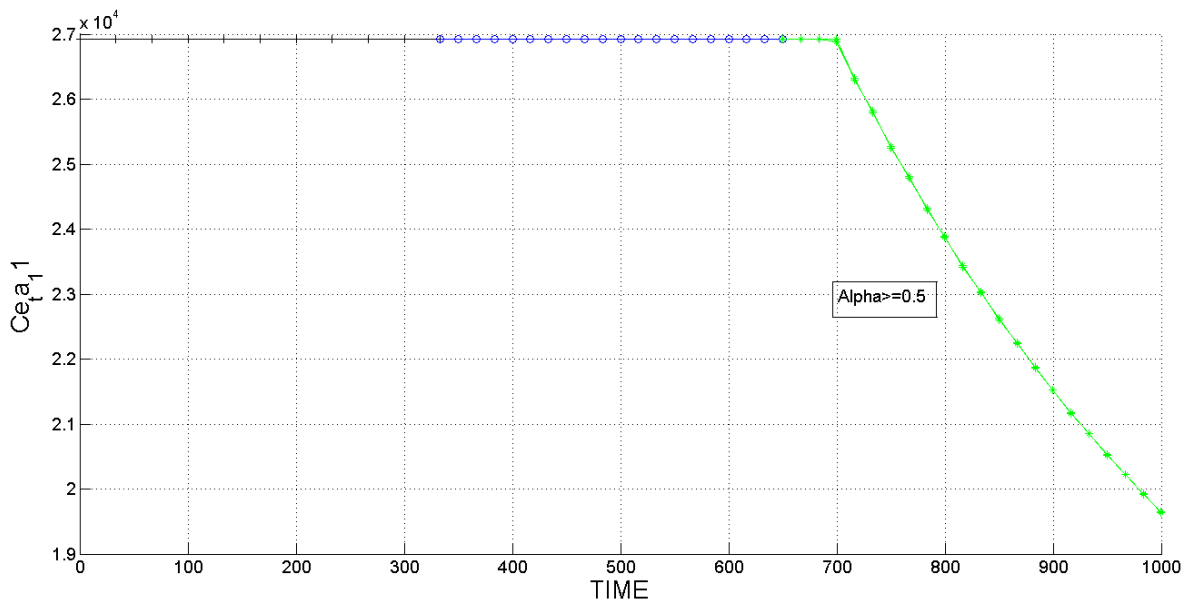
Figure 41. C11 component of tangent operator respect to \alpha when TIME-INT=1000 ( \alpha \geq 0.5 )
