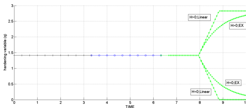
Figure 4. Hardening variable q respect to time of case A
