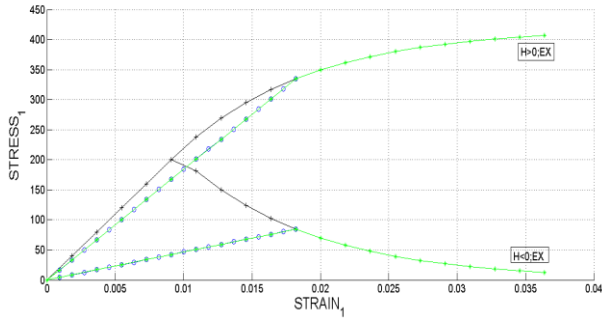
Figure 29. Strain1-Stress1 curve of case E
