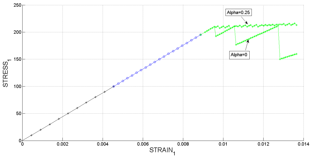
Figure 35. The Strain1-Stress1 respect to \alpha when TIME-INT=1000 ( \alpha < 0.5 )
