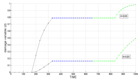
Figure 15. Damage variable respect to time of case D
