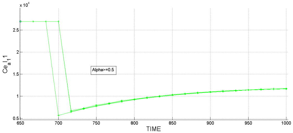
Figure 38. C11 component of algorithmic constitutive operator respect to \alpha when TIME-INT=1000 ( \alpha \geq 0.5 )
