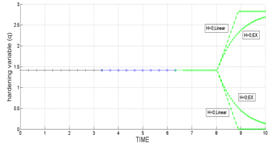
Figure 23. Hardening variable q respect to time of case B
