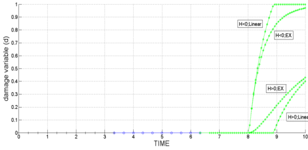
Figure 22. Damage variable respect to time of case B
