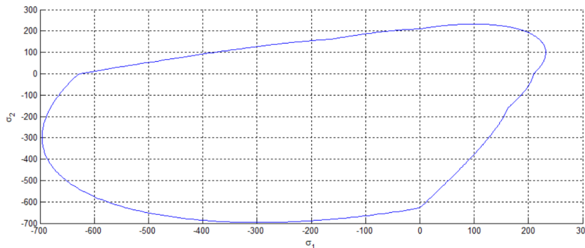
Figure 1. Non-symmetric tensile-compression damage model
