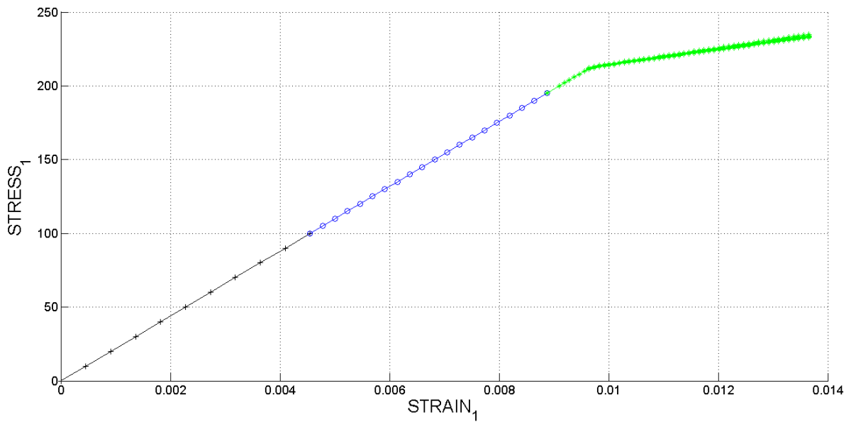
Figure 34. The Strain1-Stress1 respect to \alpha when TIME-INT=10
