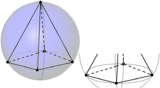
Figure 8: Five nodes on the same sphere and possible zero or almost zero volume tetrahedron (sliver) on the right.
