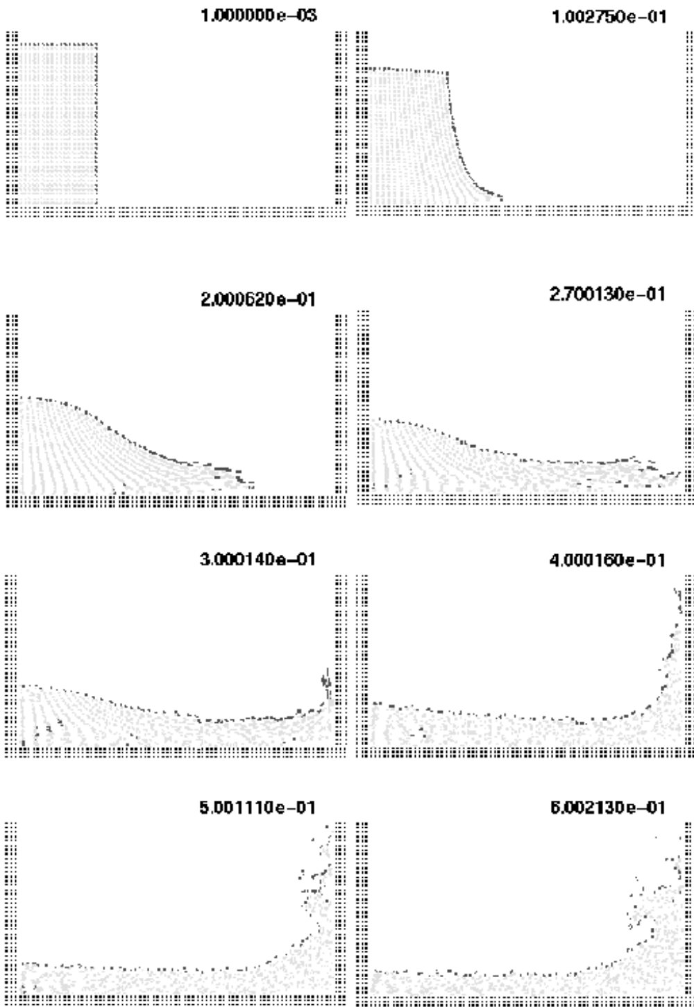
Figure 1 Water column collapse at different time steps.
