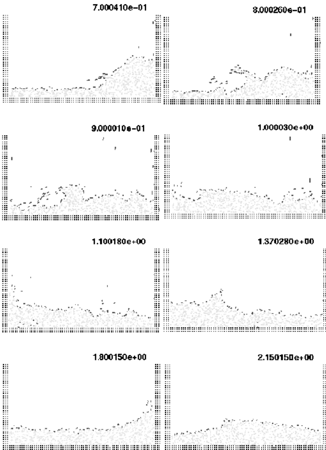
Figure 1.(Continuation):Water column collapse at different time steps.
