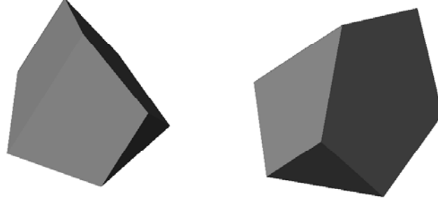
Figure 10: Eight-node polyhedron. All nodes are on the same sphere.
