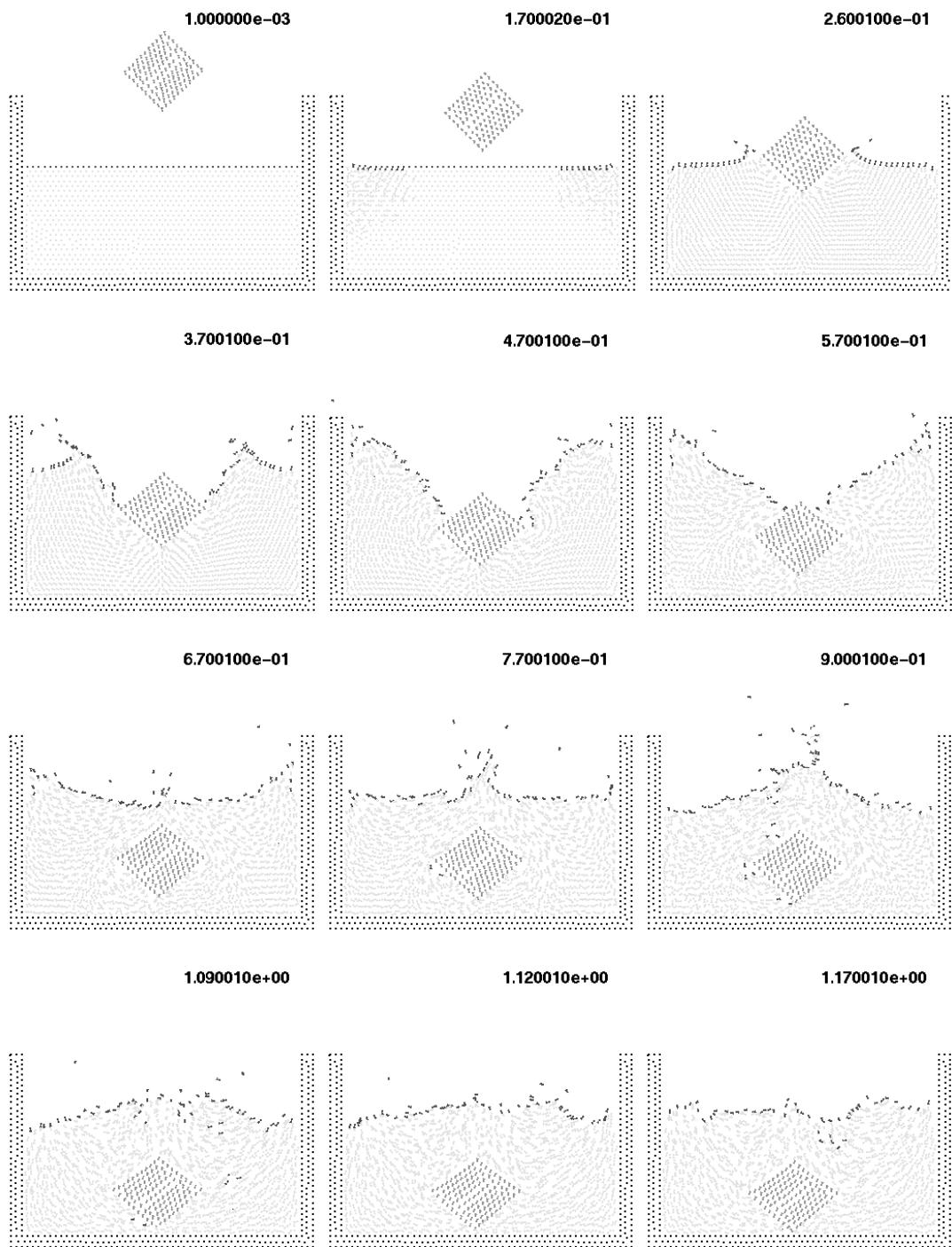
Figure 5. Solid cube falling into a recipient with water.
