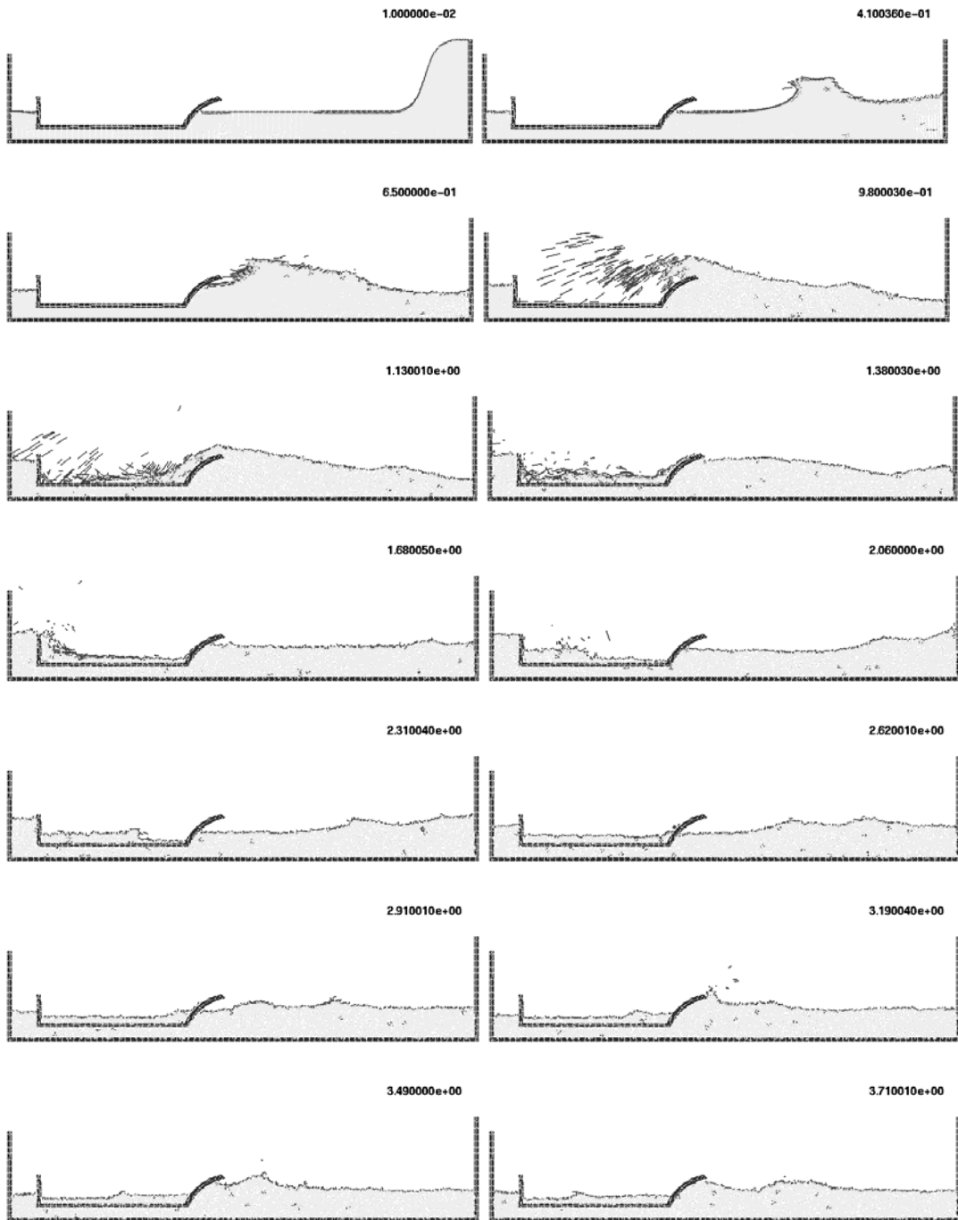
Figure 2. Fixed ship under external waves
