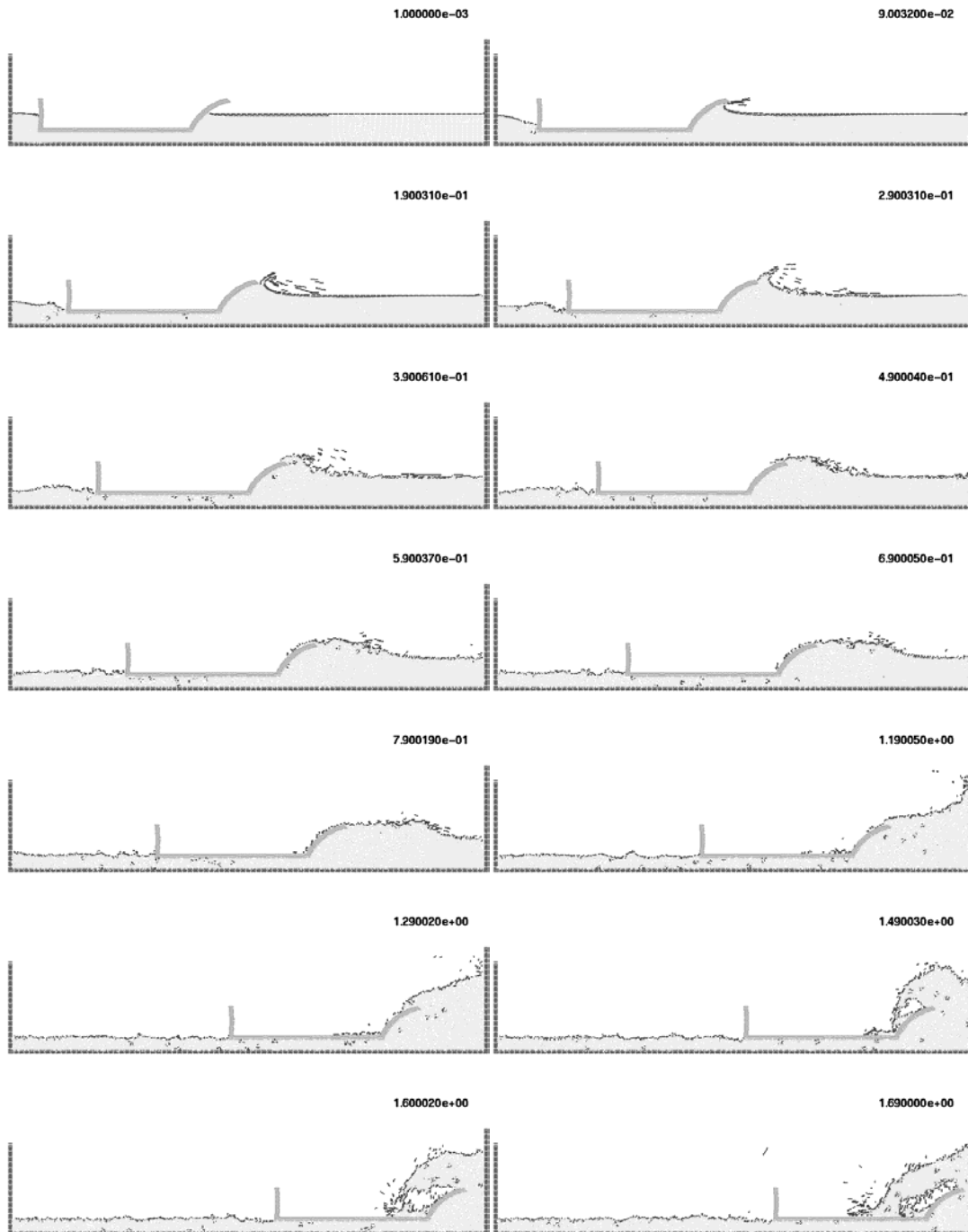
Figure 3. Moving ship with known velocity.
