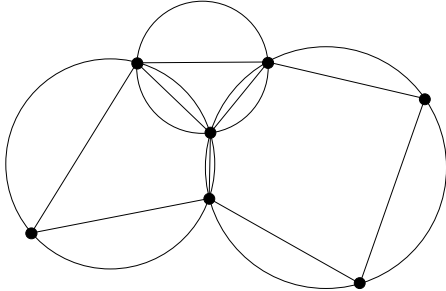
Figure 9: Two-dimensional partition in polygons. The triangle, the quadrangle and the pentagon are each inscribed on a circle
