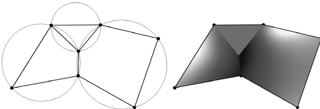
Figure 12. C^0 continuity of the shape function on a 2-D node connection.
