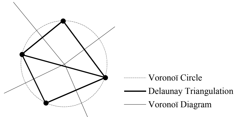
Figure 7: Voronoï diagram, Voronoï circle and Delaunay triangulation for a 4 nodes distribution in 2D.
