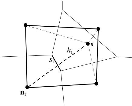
Figure 11: Four nodes and arbitrary internal point x Voronoi diagram. Shape function parameters
